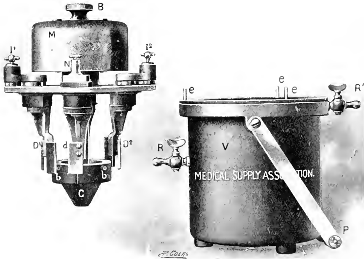
FIG. 24.—Gaiffe interrupter.
